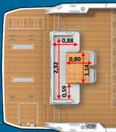
OPTION CREW CABIN U-SHAPE SEAT AFT COCKPIT
